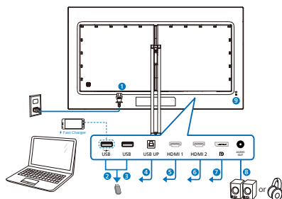
USB hub
